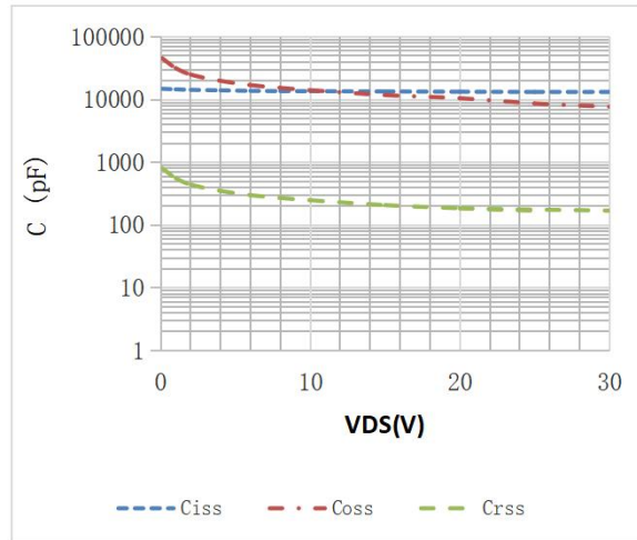
Fig.2 Capacitance Characteristics
